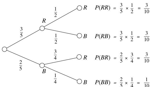
Fig. 6.2. Tree diagram with branch probabilities
